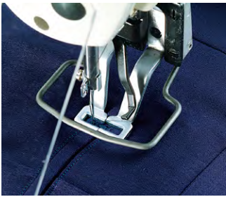
LK-1900S-S type (Bartacking pocket lip of suits)
