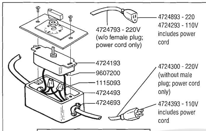
4724050 - 110V, Timer Unit Complete 4724550 - 220V, Timer Unit Complete
